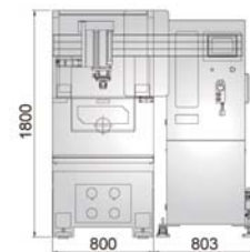
迴轉堆疊送料 Rotary Stocker
