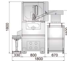
滑軌氣壓送料 Sliding Feeder
